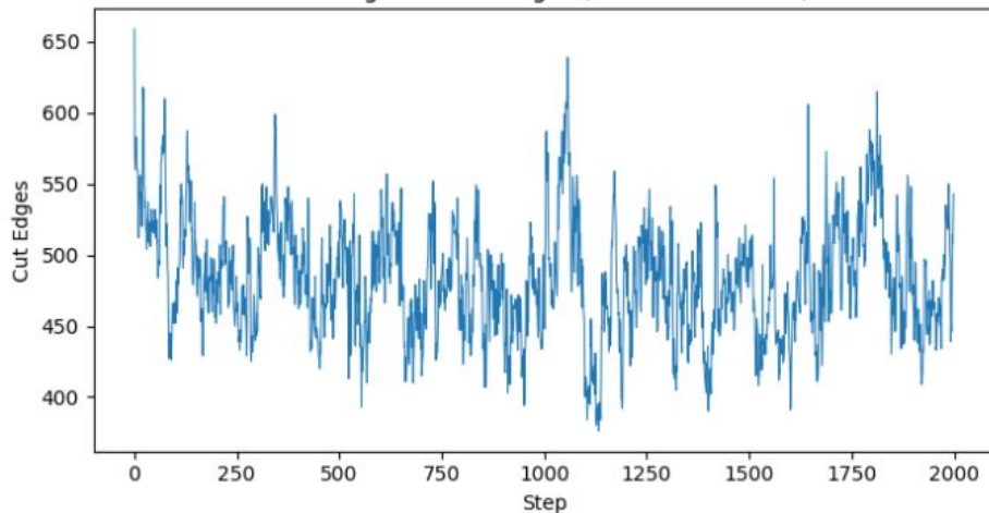
Convergence: Cut Edges (2024 Presidential)
