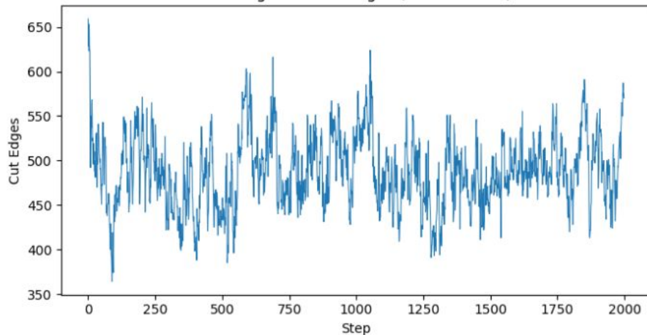
Convergence: Cut Edges (2024 Senate)
